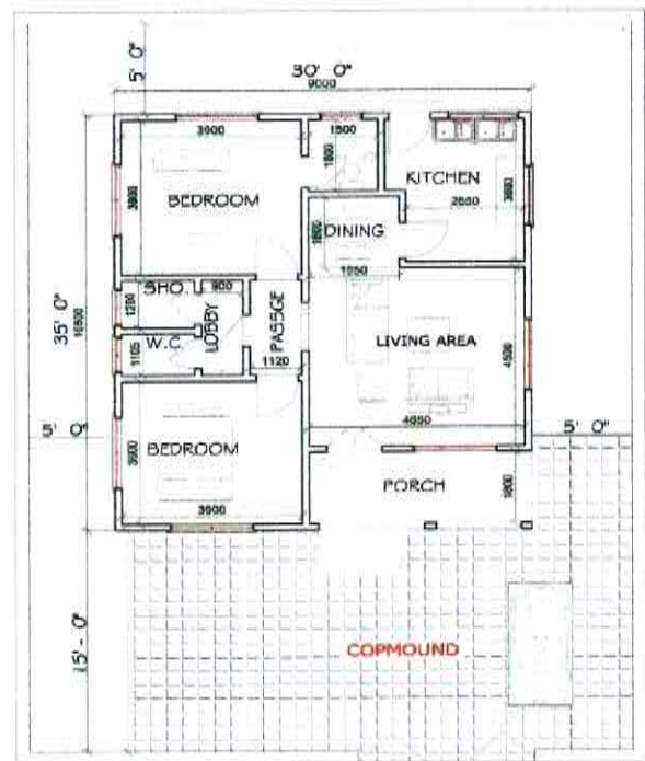
2-BEDROOM FLAT PLOT SIZE 40X55.
