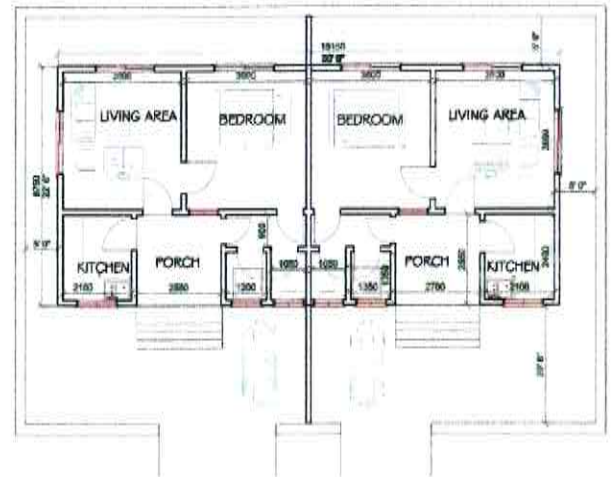
ONE BEDROOM SEMI-DETACH PLOT SIZE 40X60.
