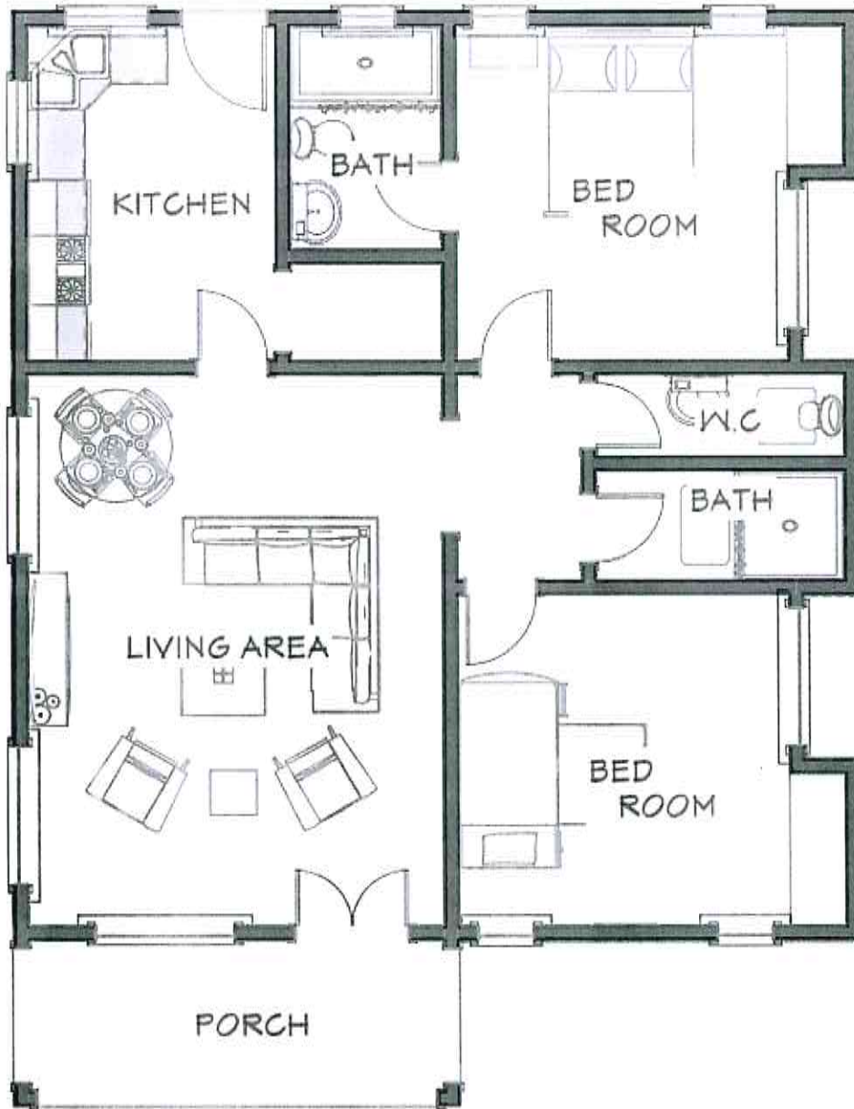
2 BEDROOM STANDARD
